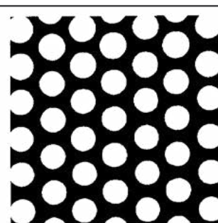
R5 T7 45% - 5mm hole
