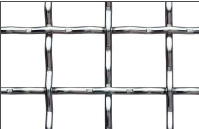
22.4mm Aperture x 3.15mm Wire Dia. / Intercripped
