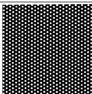
R0.8 T1.5 25% - 0.8mm hole
