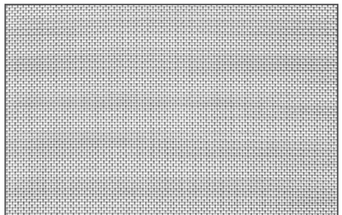
0.415mm Aperture x 0.22mm Wire Dia.
