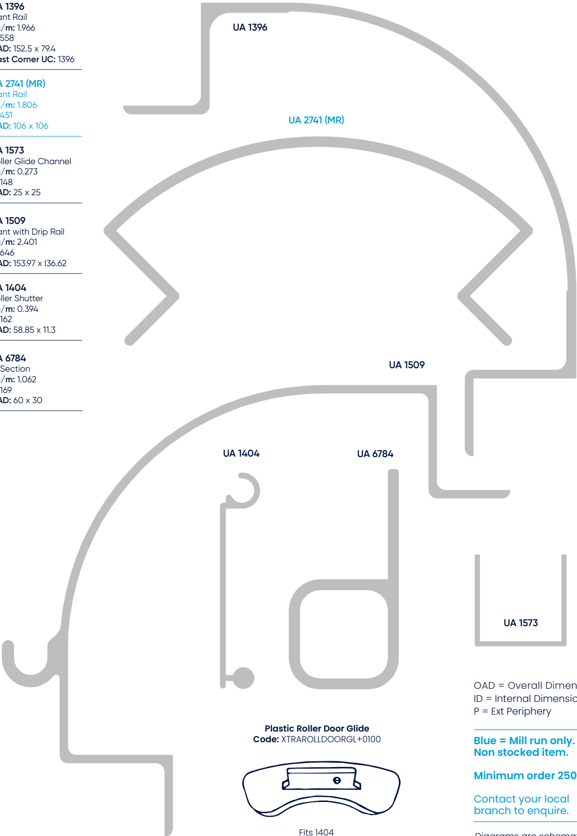
Fits 1404 Each end of every second shutter Minimum inside radius bend of 150mm
